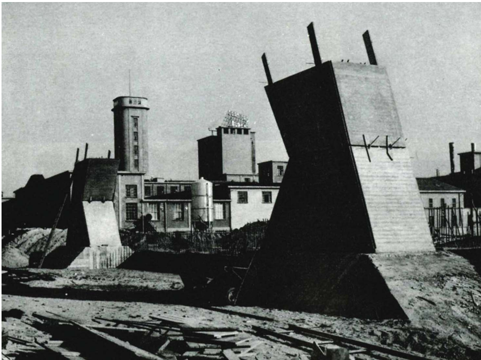
Figure 17. Photograph of the Burgo Paper Mill, detail of the reinforced concrete support [MAXXI Architettura, Rome, Italy] (color figure available online).
