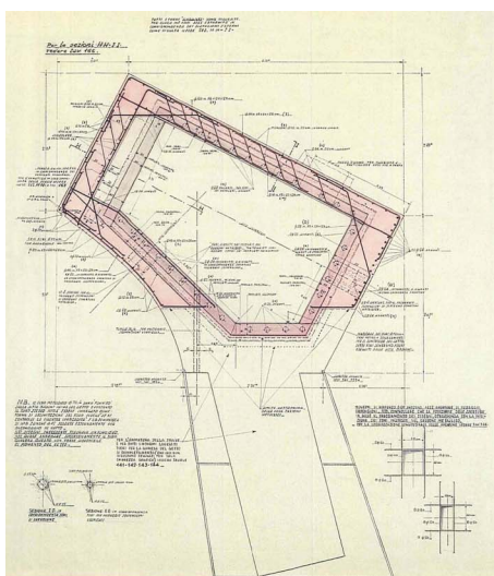
Figure 19. Diagram of a cross section (the reinforcement around the steel box, red in online files) and a photograph of the positioning of the hybrid connection between the support and the chain, the steel box [CSAC, Parma, Italy; Burgo, Mantua, Italy] (color figure available online).
