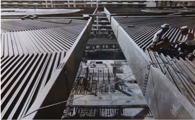
Figure 14. Photograph of the Palace of Labour, the original roof in steel, removed in 1963 [Courtesy of PlannING, Bologna, Italy] (color figure available online).
