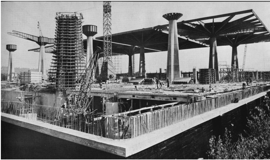
Figure 9. Photograph of the Palace of Labour, in construction [MAXXI Architettura, Rome, Italy].
