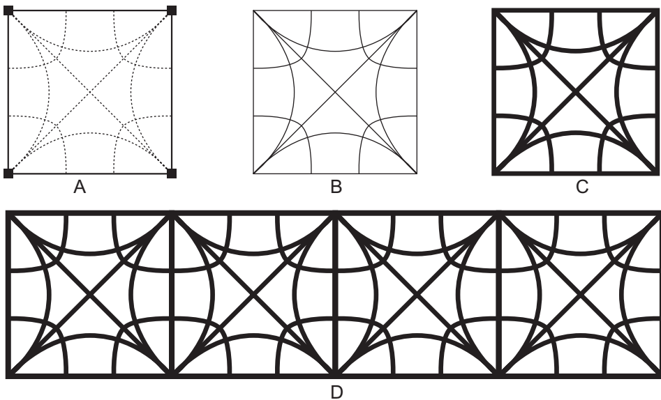
Figure 10. Diagrams of the isostatics (A), the reinforcement lines (B), the definition of a ribbed slab (C), and the final ceiling pattern (D) [Manuel Cresciani's personal archive].
