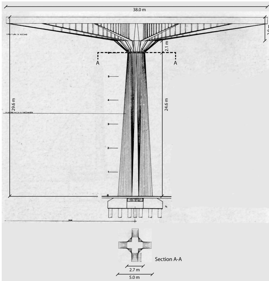
Figure 7. Diagram of the elevation and section of the column [CSAC, Parma, Italy].
