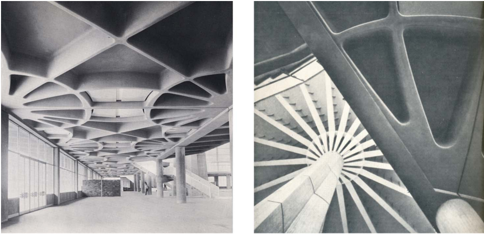
Figure 11. Photographs of the Palace of Labour, the isostatic floor [MAXXI Architettura, Rome, Italy] (color figure available online).
